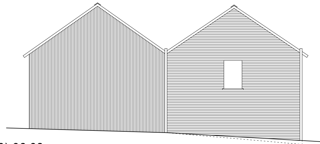
AL (0) 06.03 NORTH ELEVATION BUILDING 2 As Existing 1:100 SCALE
