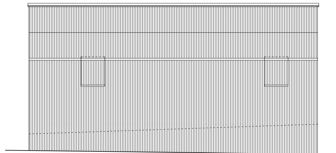
AL (0) 06.05 WEST ELEVATION BUILDING 2 As Existing 1:100 SCALE
