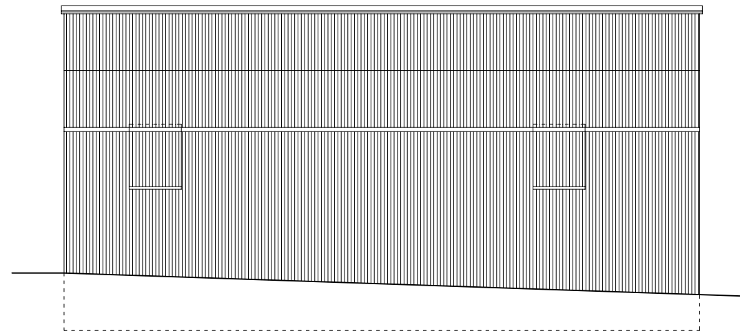
AL (0) 06.04 EAST ELEVATION BUILDING 2 As Existing 1:100 SCALE
