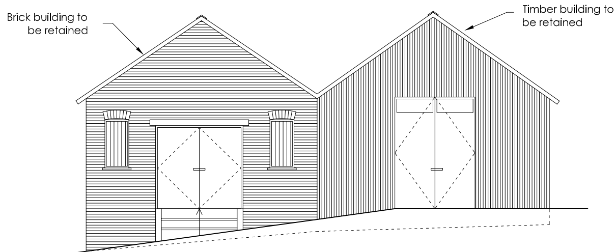
AL (0) 06.02 SOUTH ELEVATION BUILDING 2 As Existing 1:100 SCALE
